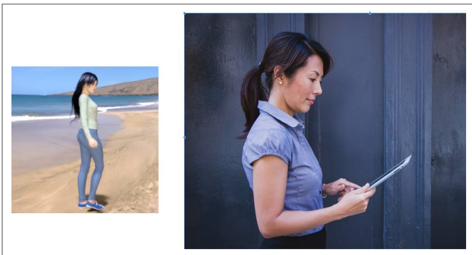
Figure 3-11. Dataset similarities
